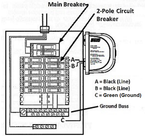
Service Panel Installation
