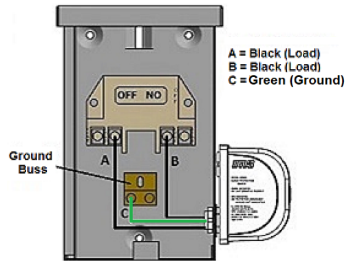
HVAC Disconnect Box 120/240Vac three wire w/ground Installation
