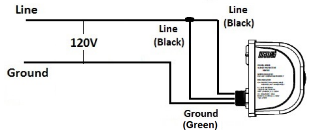
120Vac two wire single phase w/ground Installation
